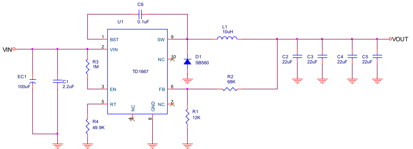
Figure2 Application Circuit, 5V Output
