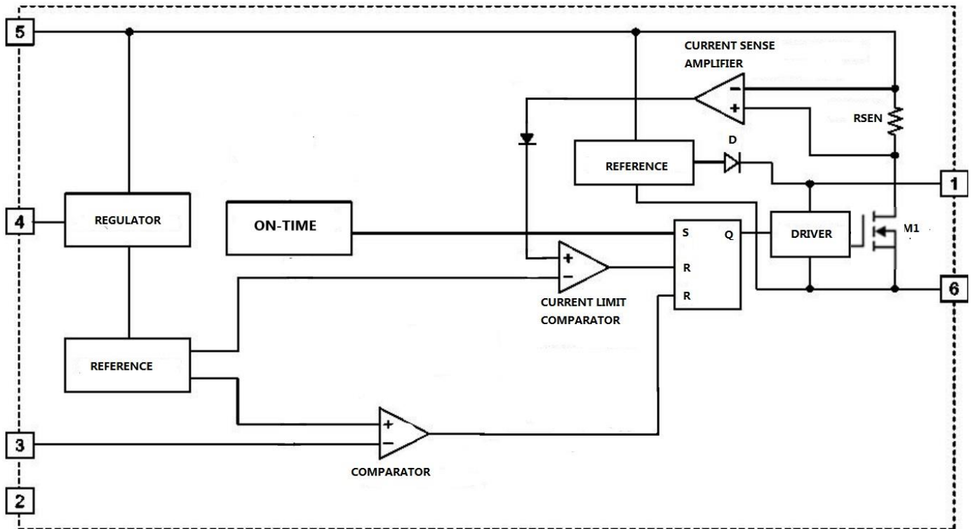
Figure1 Function Block Diagram of TD1558B
