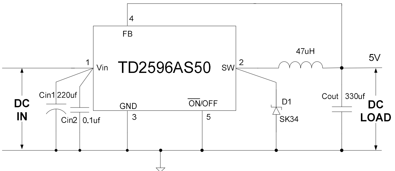
Figure 4 Typical Application of TD2596AS50
