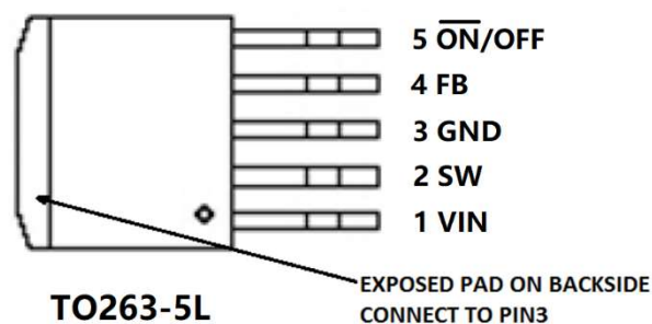
Figure1 Pin Configuration of TD2596A(Top View)
