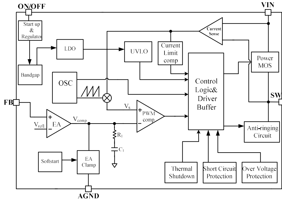
Figure 2 Function Block Diagram of TD2596A
