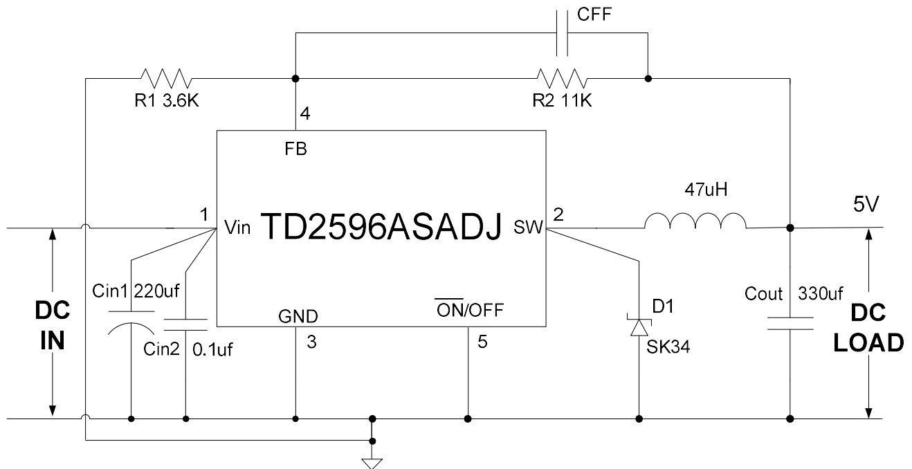
Figure 3 Typical Application of TD2596ASADJ
