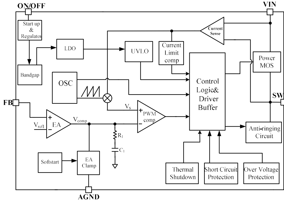
Figure 3 Function Block Diagram of TD1433A
