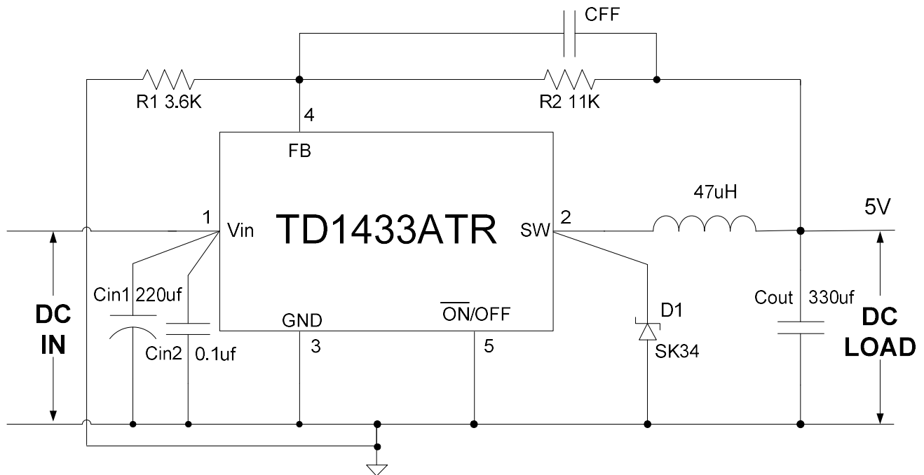
Figure 4 Typical Application of TD1433ATR
