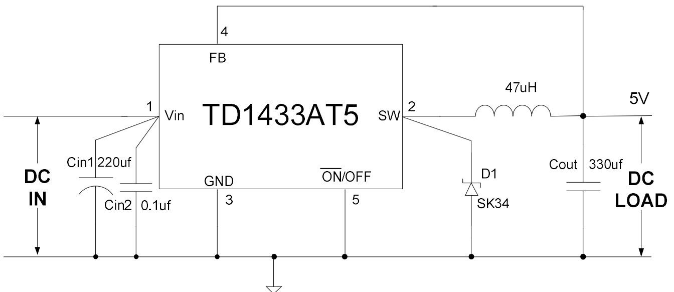
Figure 5 Typical Application of TD1433AT5
