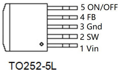
Figure2 Pin Configuration of TD1433A(Top View)
