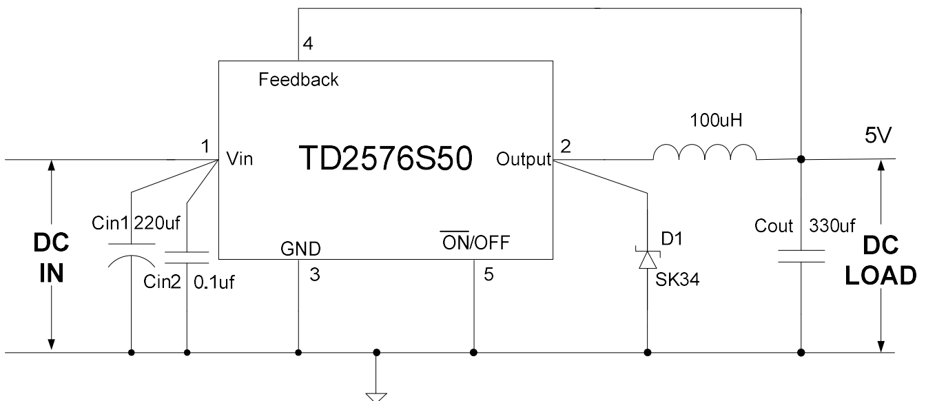
Figure 4 Typical Application of TD2576S50
