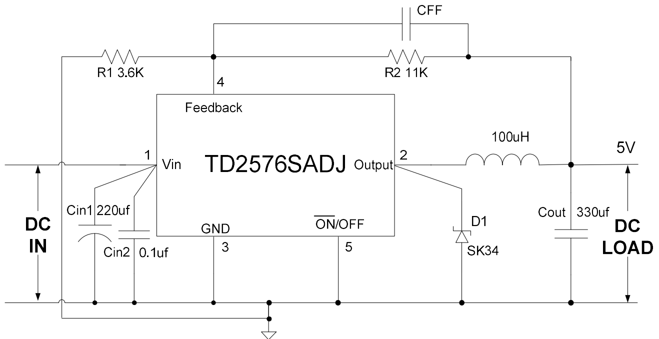
Figure 3 Typical Application of TD2576SADJ
