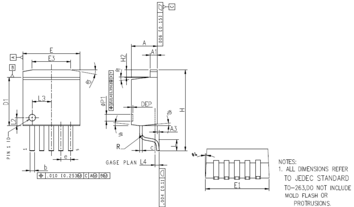
COMMON DIMENSIONS
