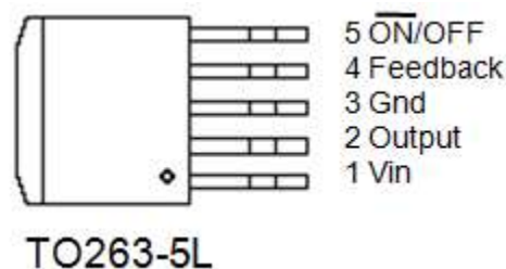
Figure1 Pin Configuration of TD2576(Top View)
