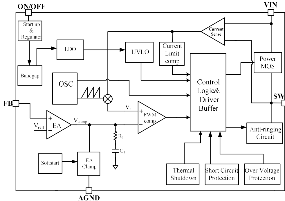
Figure 2 Function Block Diagram of TD2576
