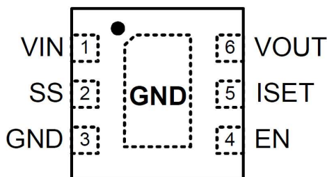
TDFN2X2-6(Top View)
