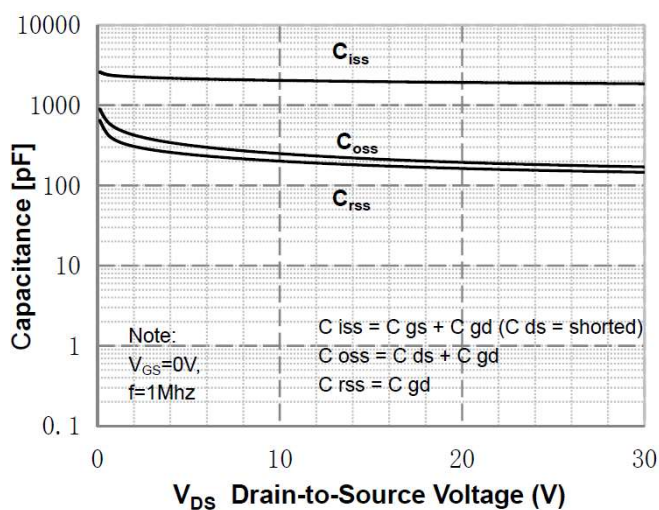
Figure 5. Capacitance Characteristics
