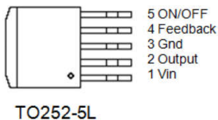
Figure2 Pin Configuration of TD1463(Top View)
