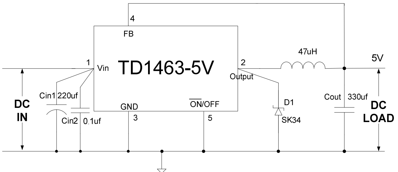
Figure 5 Typical Application of TD1463T5
