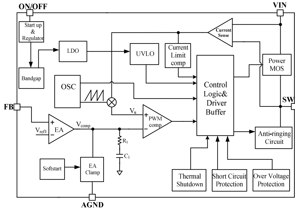
Figure 3 Function Block Diagram of TD1463
