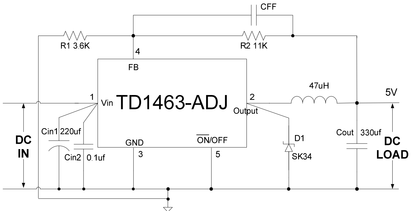
Figure 4 Typical Application of TD1463TR
