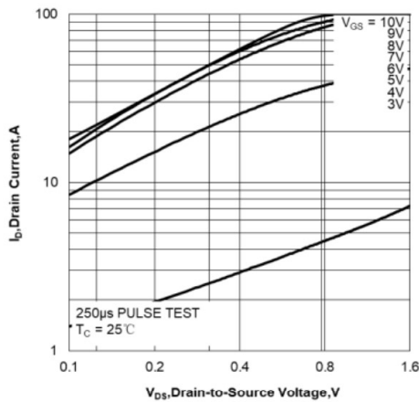
Figure 1. Output Characteristics
