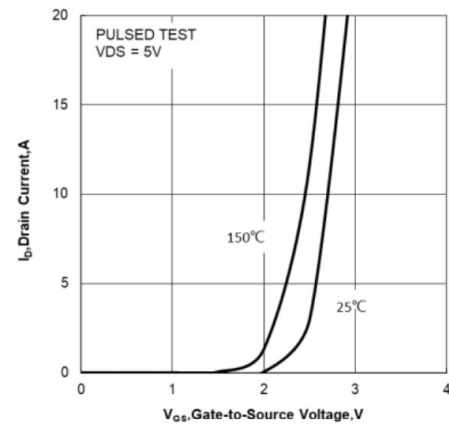
Figure 2. Transfer Characteristics
