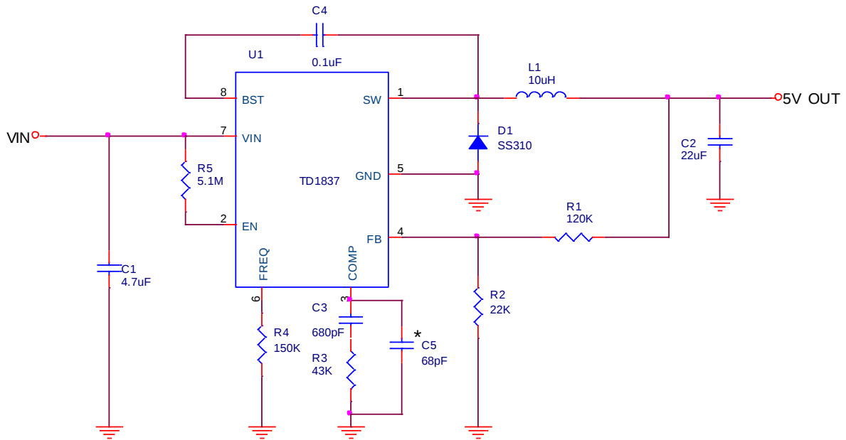
Figure2 Vin&lt;64V, 5V Output Typical Application Schematic
