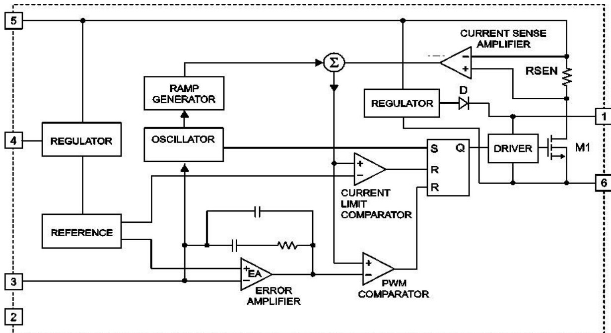
Figure1 Function Block Diagram of TD1605
