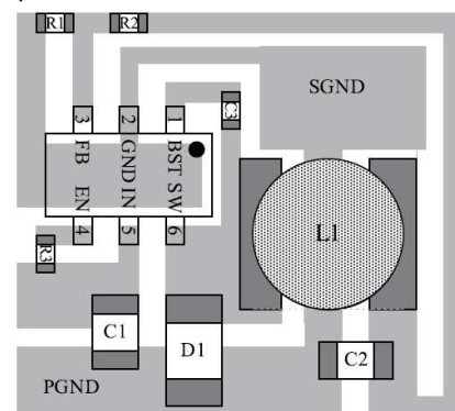
Figure 2: PCB Layout
