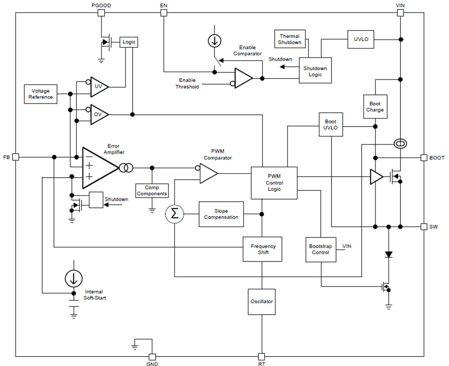
Figure1 Function Block Diagram of TD1663A
