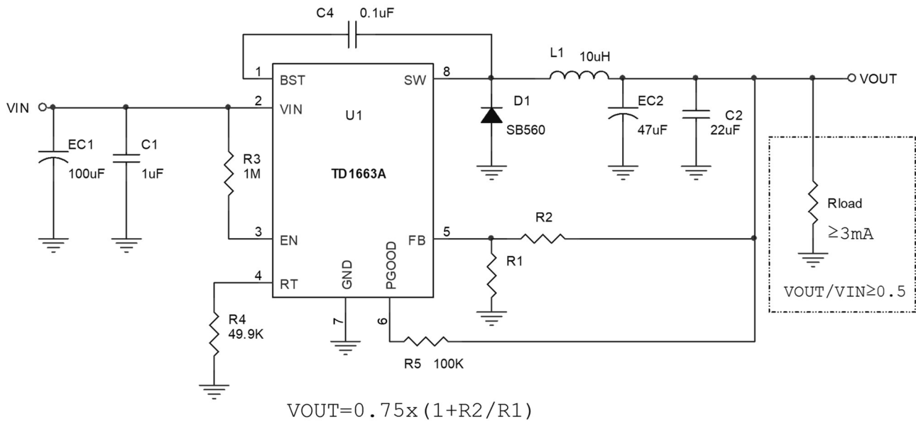
Figure2 Application Circuit
