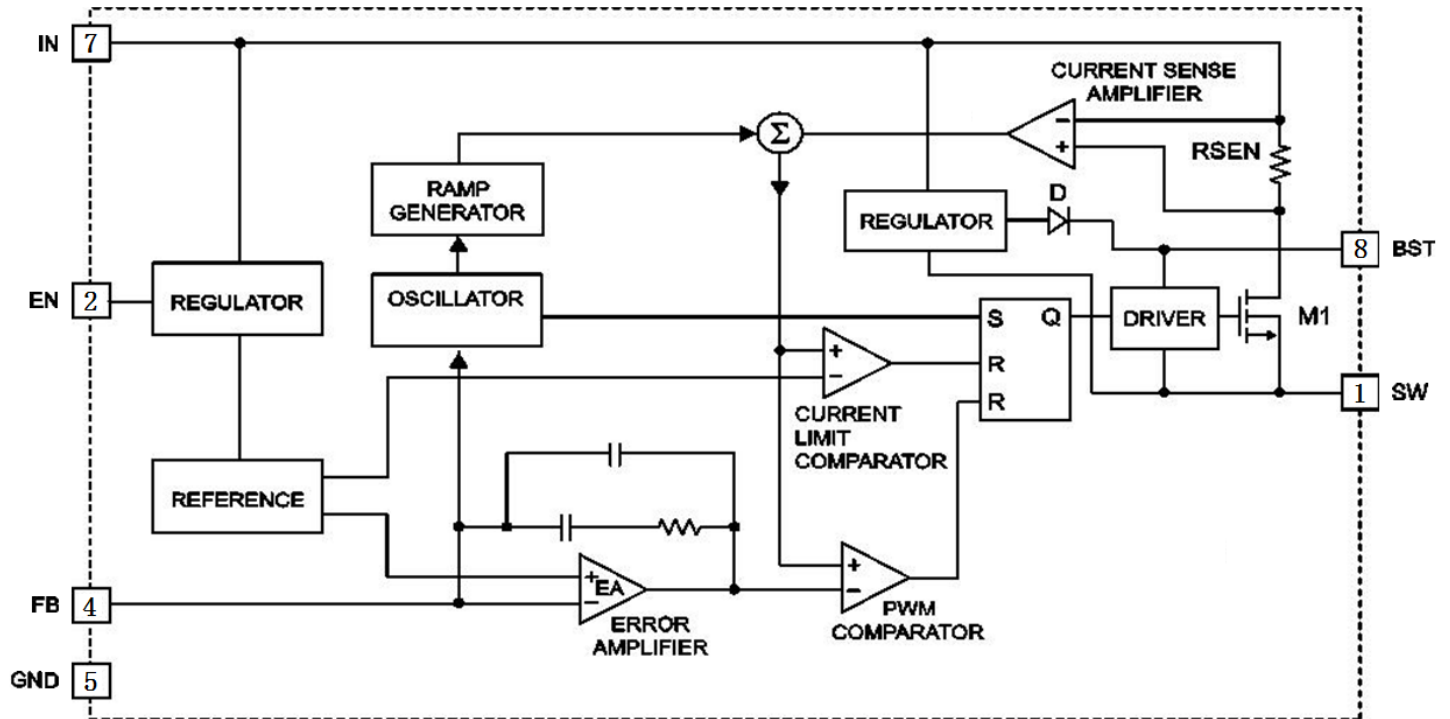
Figure1 Function Block Diagram of TD1688
