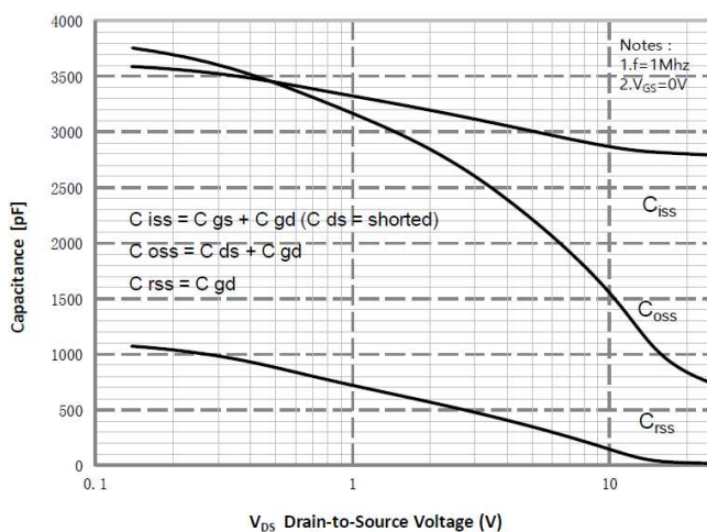
Figure 5. Capacitance Characteristics
