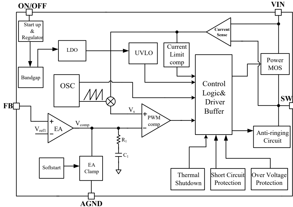
Figure 2 Function Block Diagram of TD1509HV
