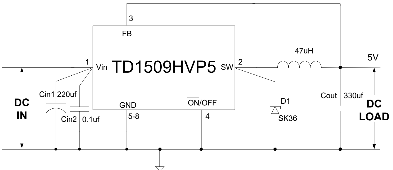
Figure 4 Typical Application of TD1509HVP5
