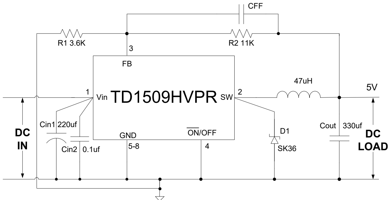
Figure 3 Typical Application of TD1509HVPR
