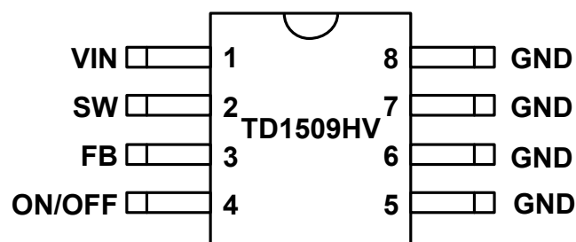
Figure1 Pin Configuration of TD1509HV(Top View)
