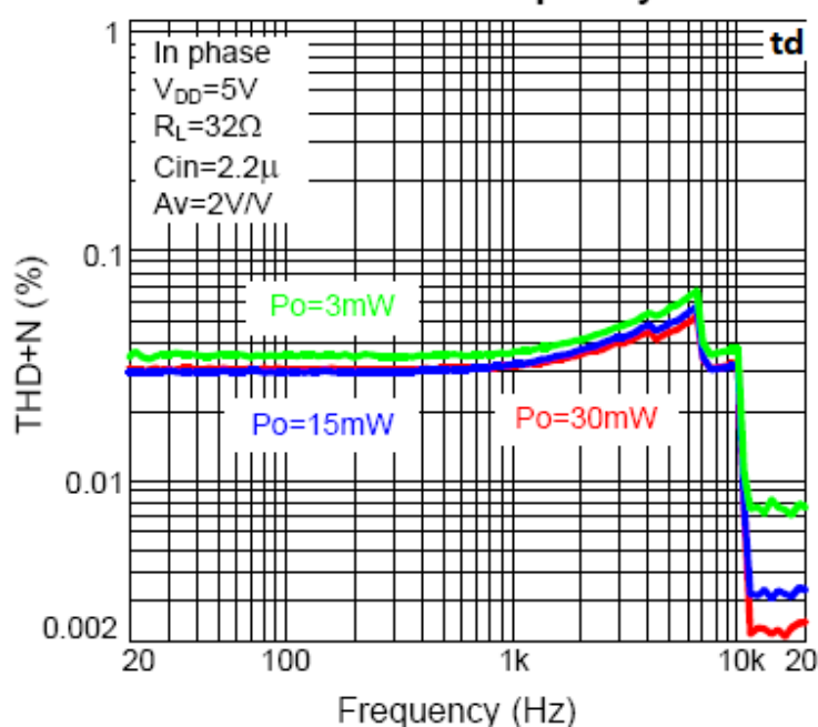
THD+N vs. Frequency
