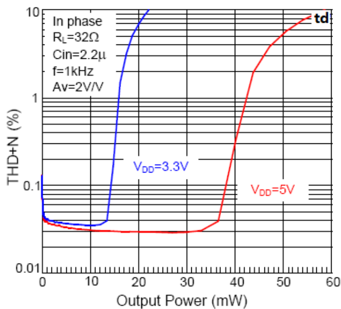
THD+N vs. Output Power
