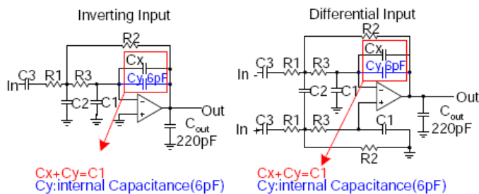
Figure 3. Second-Order Active Low-Pass Filter
