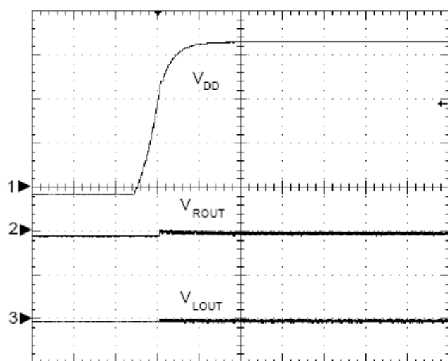
Output Transient at Power On
