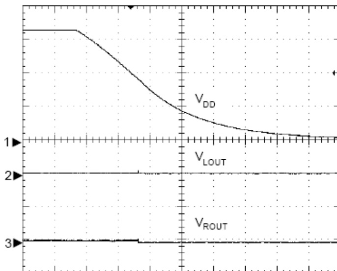
Output Transient at Power Off
