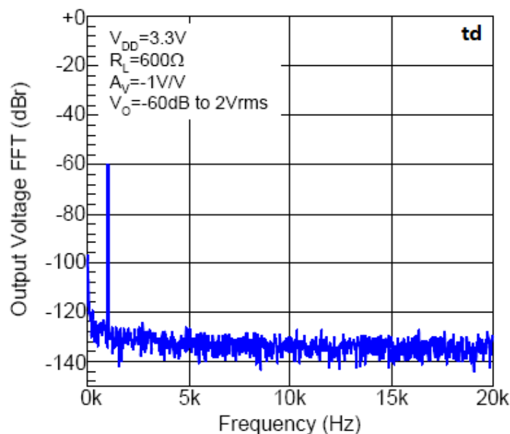
Output Voltage FFT vs. Frequency
