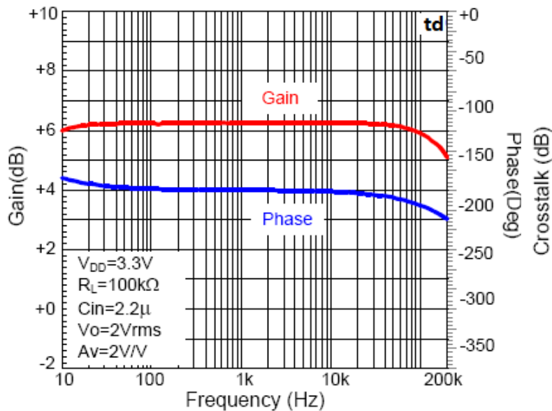
Frequency Response
