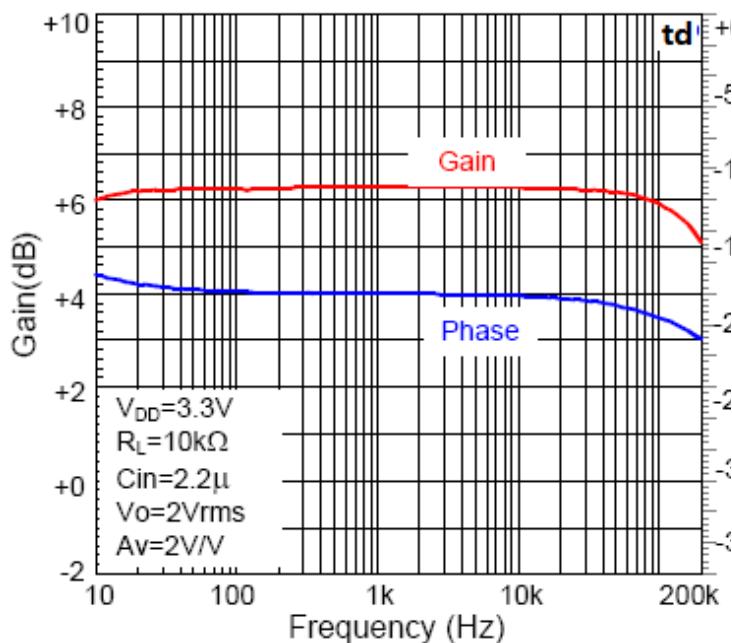
Frequency Response
