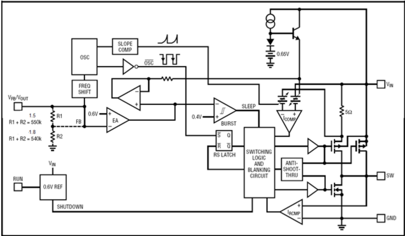
Figure2:Functional Block Diagram of TD6811B
