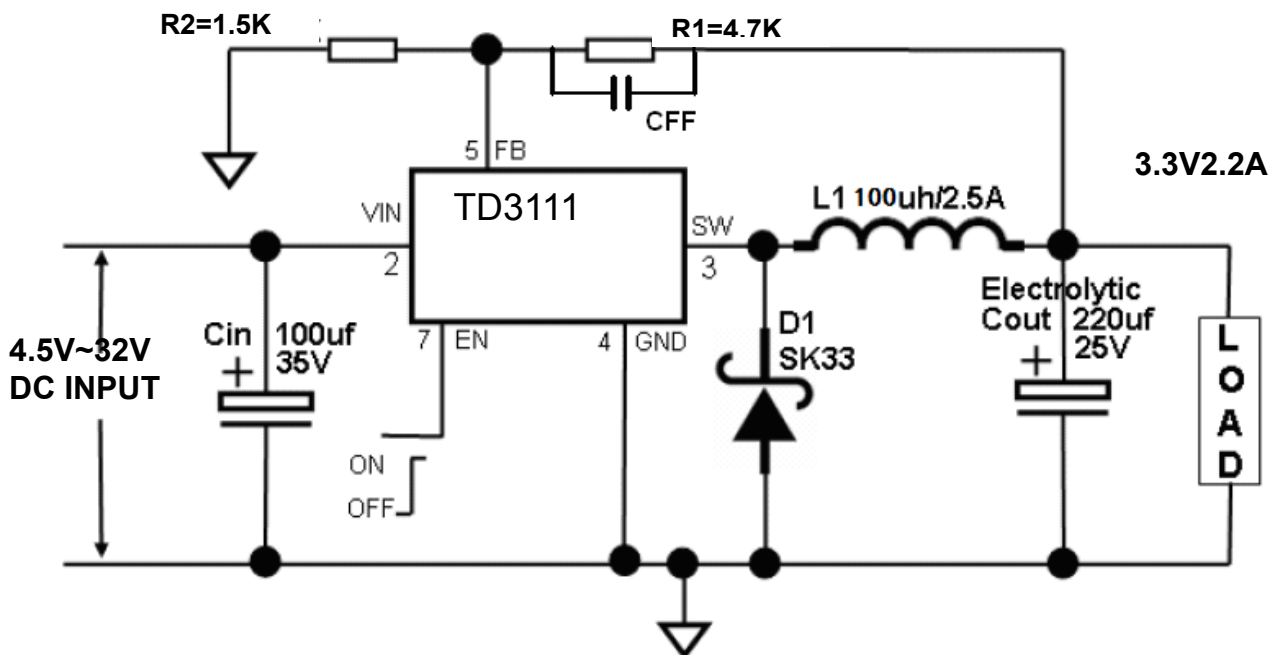
Fig9. TD3111 Typical Application Circuit @ 3.3V/2.2A
